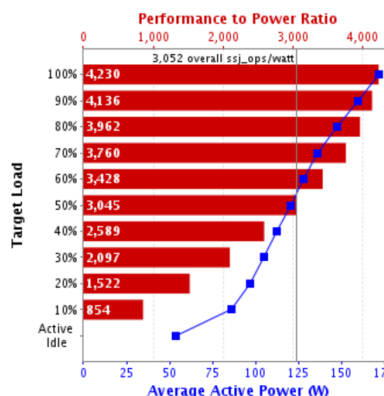
Servers consume a significant amount of power when they are idle, often more than 50% of peak power. As shown above, moving from 10% load to 50% load delivers 5x the performance for 40% more power.
